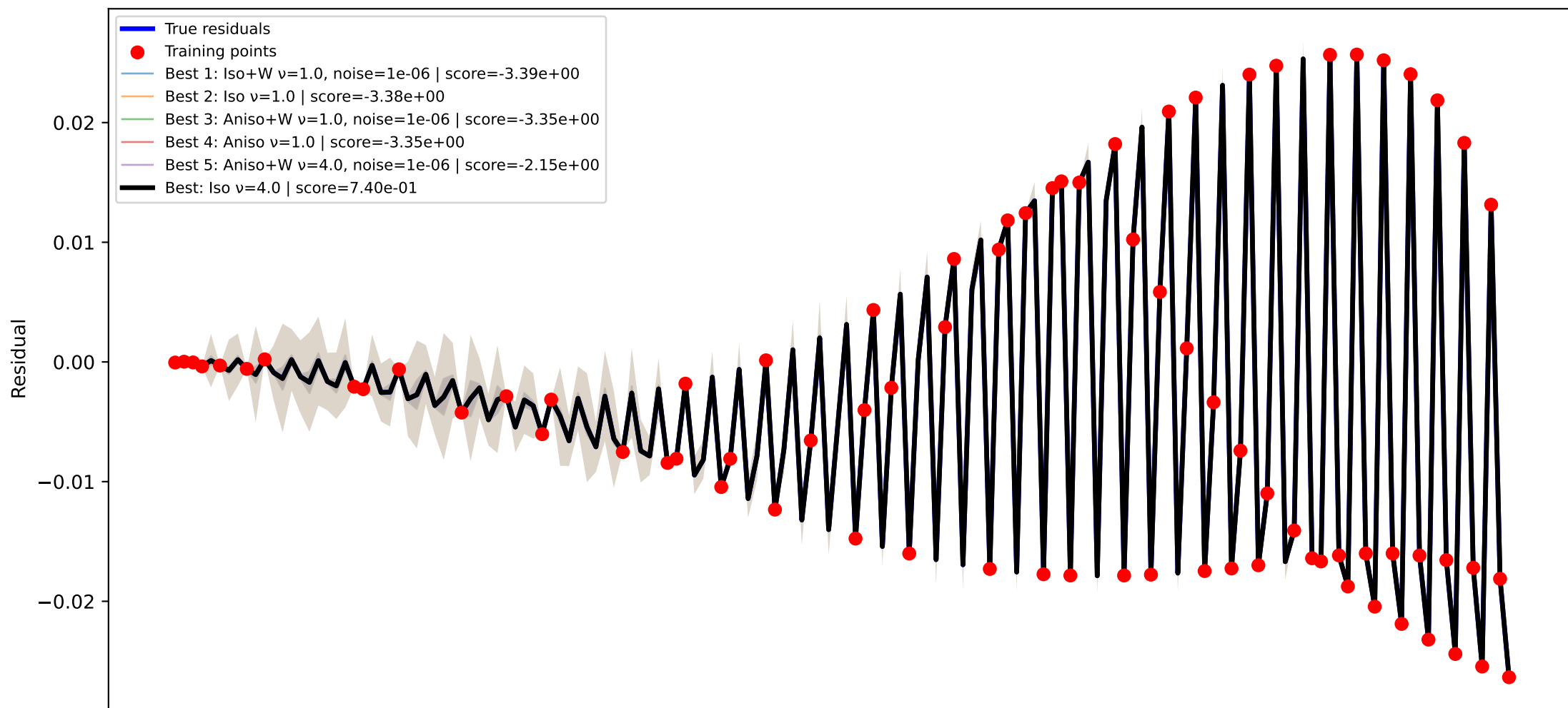
GPR kernel comparison node=40 RMSE=5.966e-06, train RMSE=2.180e-09
